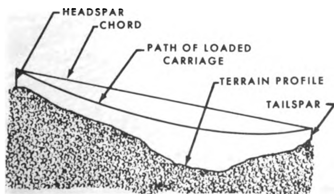
Figure 7-27. Typical profile plot of a grapple yarding layout.
